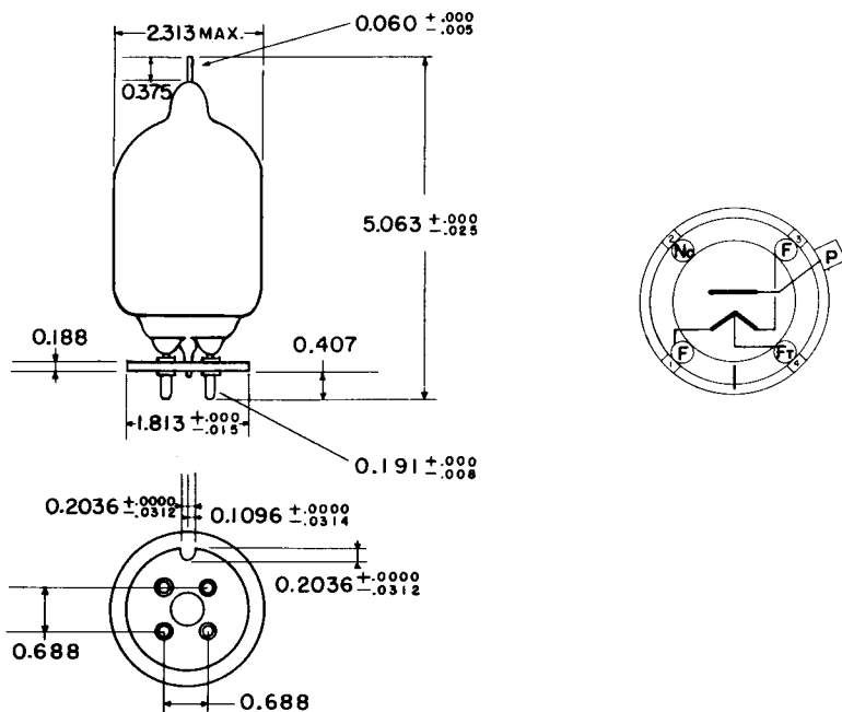
TUBE DIMENSIONS
